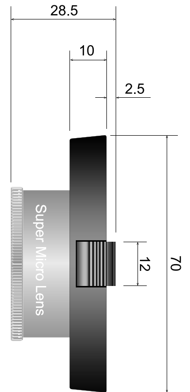
Macro lens + UAC3500 Universal Adapter
