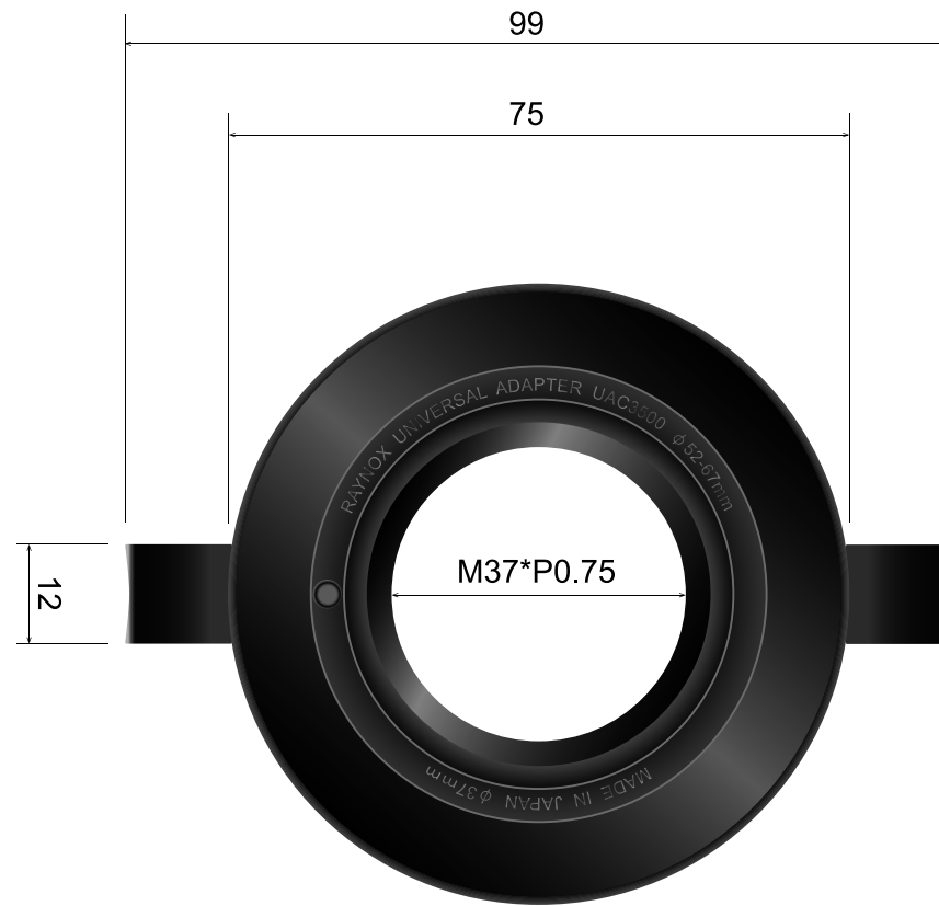
UAC3500 Universal Adapter
