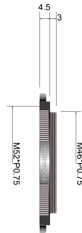
RA5246B Adapter ring
