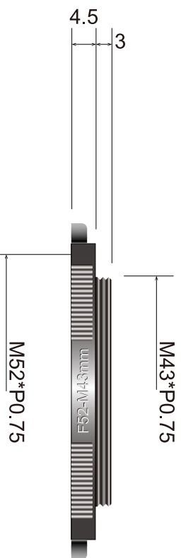
RA5243B Adapter ring
