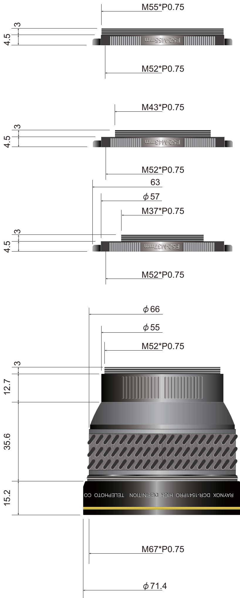
RA5237B Adapter ring
