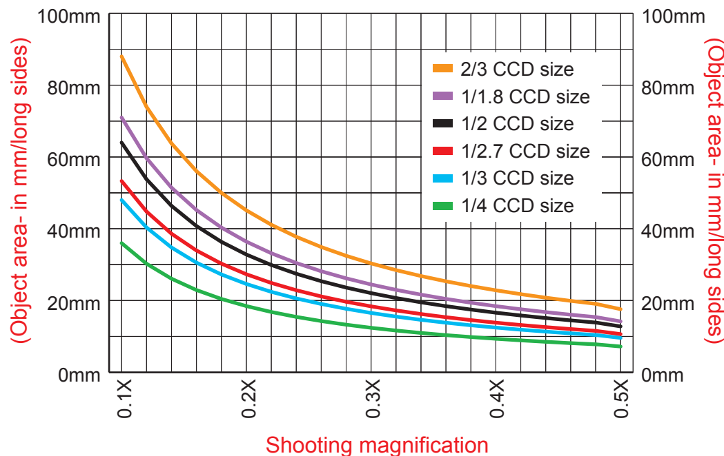
Interrelation between Shooting magnification and object area
