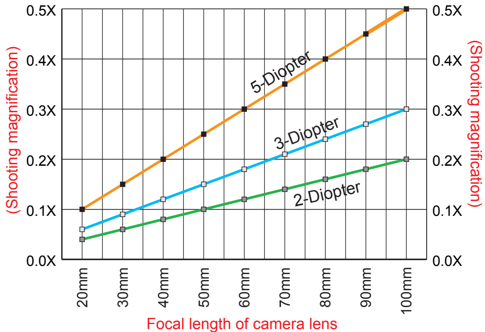
Interrelation between diopter and shooting magnification
